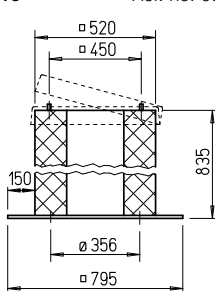
Hood silencer HSDV 315
