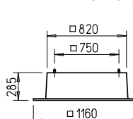
Flat roof base FDS 560
