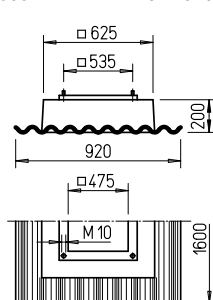
Base silencer, hinged SSD 355
