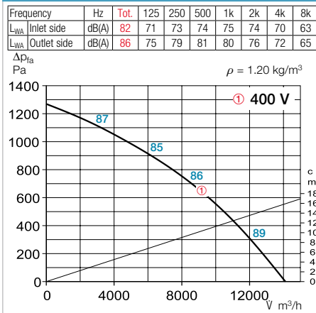
Performance curve VDD 560/4
