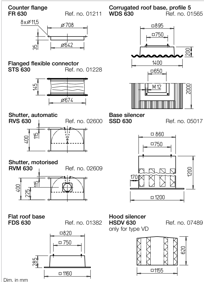
Dimensions Accessories for RD EC 630 / VD EC 630
