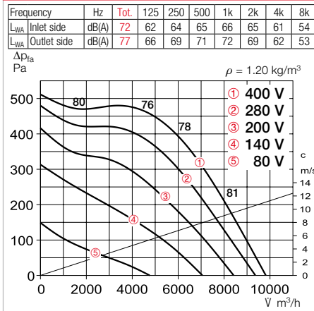
Performance curves RDD 560/6
