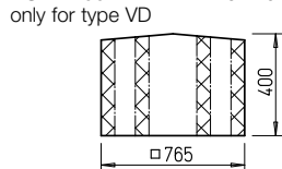
Hood silencer HSDV 400
