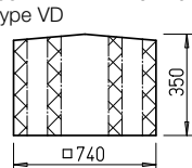
Hood silencer HSDV 355
