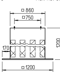
Base silencer SSD 560
