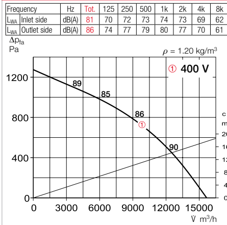
Performance curve RDD 560/4
