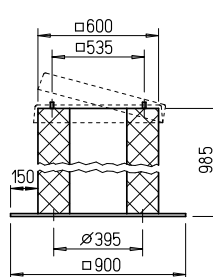
Hood silencer HSDV 355
