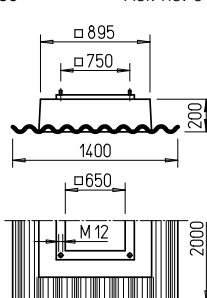
Base silencer SSD 560
