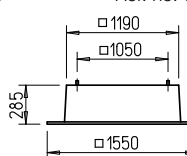
Flat roof base FDS 710
