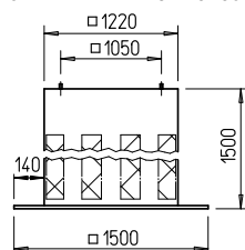
Base silencer SSD 710
