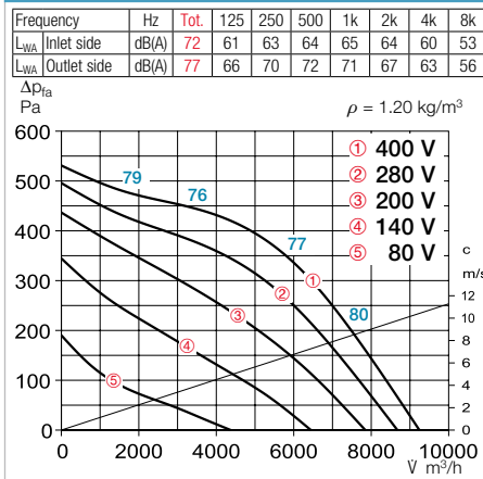
Performance curves VDD 560/6
