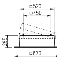
Flat roof base, hinged FDS 315
