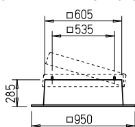
Flat roof base, hinged FDS 355
